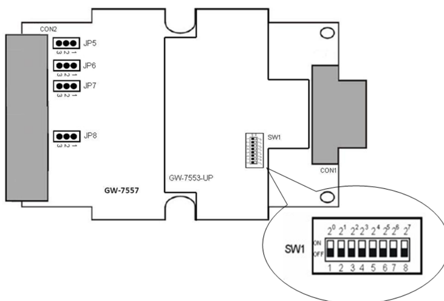
Figure 11 DIP switch
