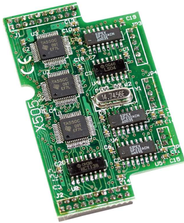
X505 3-Port RS-232 (5-Pin)
