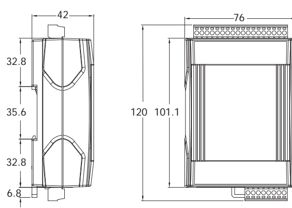
ET-7200/PET-7200 Series
